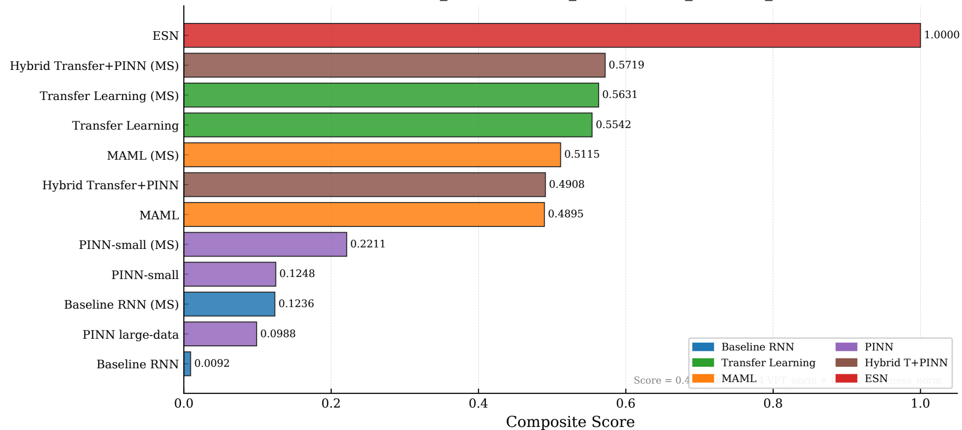
Lorenz — Three-Metric Composite Leaderboard \text{Score} = 0.4 \cdot R^2_{\text{norm}} + 0.4 \cdot \text{VPT}_{\text{norm}} + 0.2 \cdot D_2_{\text{closeness}_{\text{norm}}}
